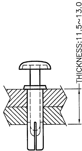
MOUNTING HOLE: \phi 4.0 DIAGRAM
