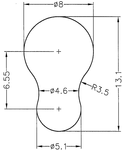
MOUNTING HOLE
