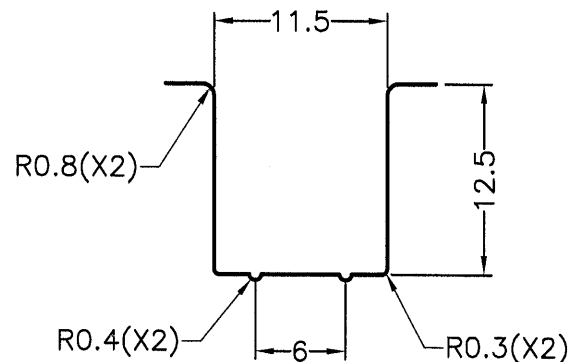
MOUNTING HOLE CHASSIS THICKNESS 0.8mm
