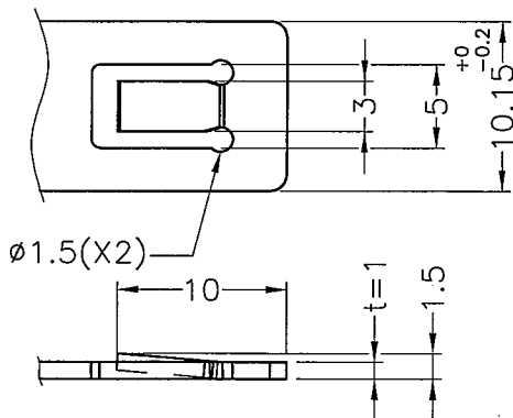
ASSEMBLY PART
