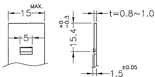
ASSEMBLY PART (裝配件尺寸, 僅供參考)
