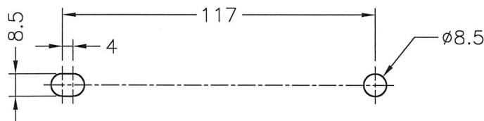
MOUNTING HOLE (RECOMMEND FOR REFERENCE ONLY)
