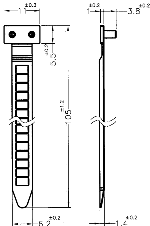
CABLE TIES
