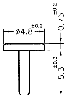
CABLE CLAMP
