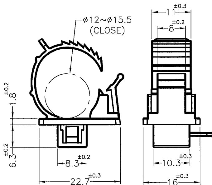
CABLE CLAMP
