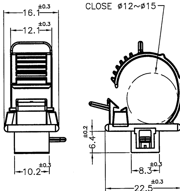
CABLE CLAMP
