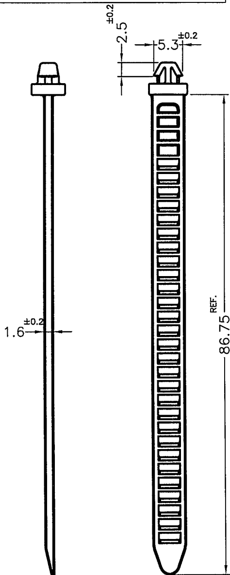
CABLE TIES
