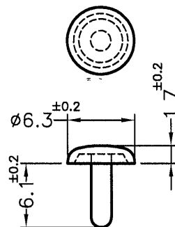
SR3.5-5B SCALE 2:1
