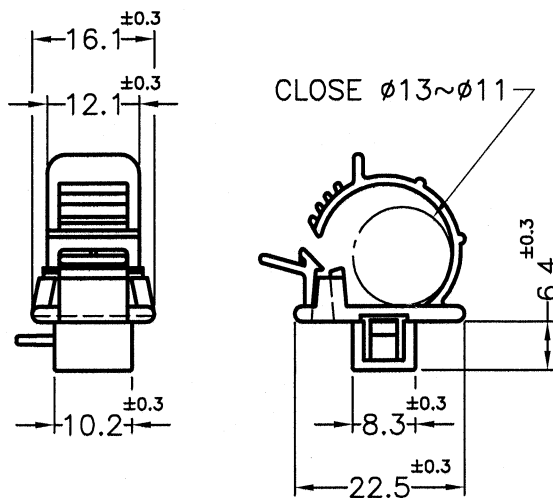
CABLE CLAMP
