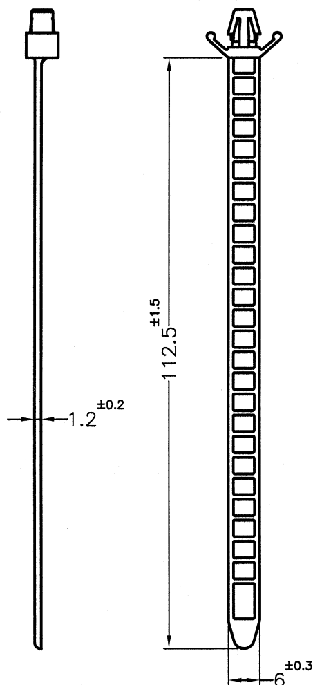
CABLE TIES
