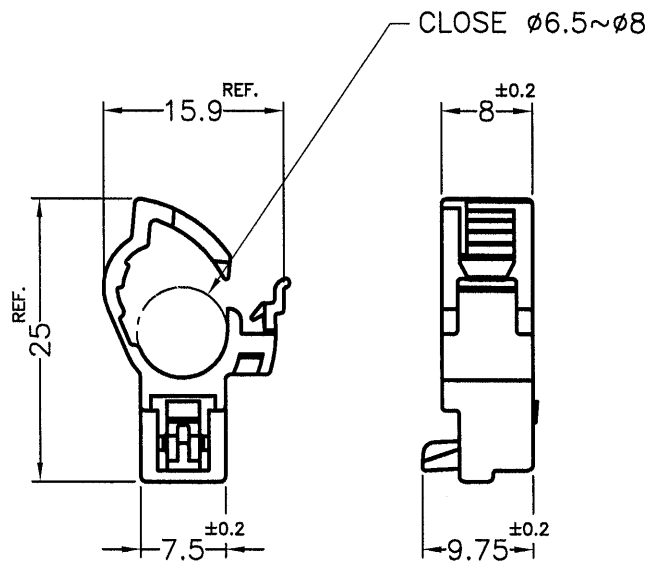
CABLE CLAMP
