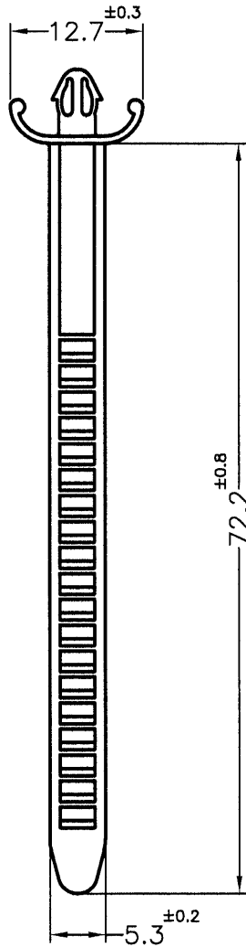
CABLE TIES
