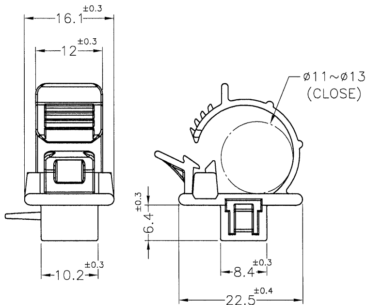
CABLE CLAMP
