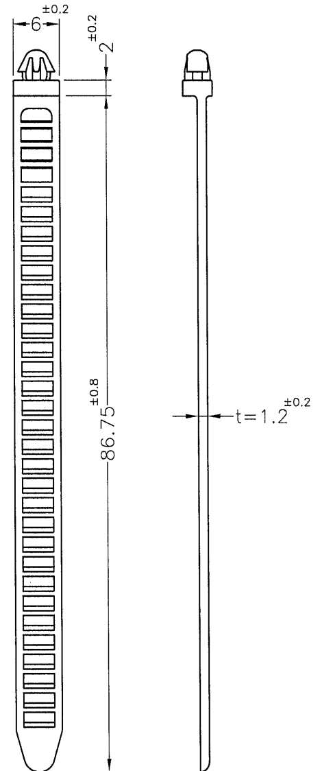
CABLE TIES
