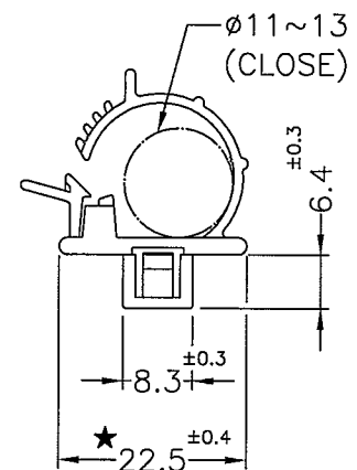
CABLE CLAMP
