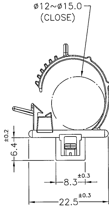
CABLE CLAMP
