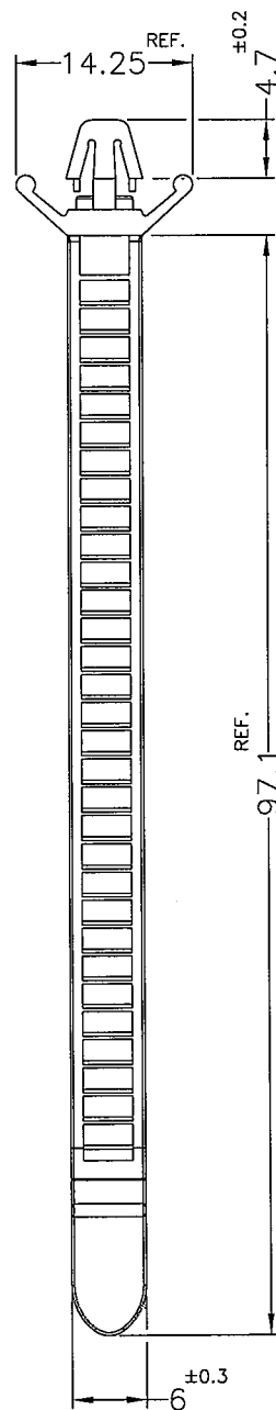
CABLE TIES
