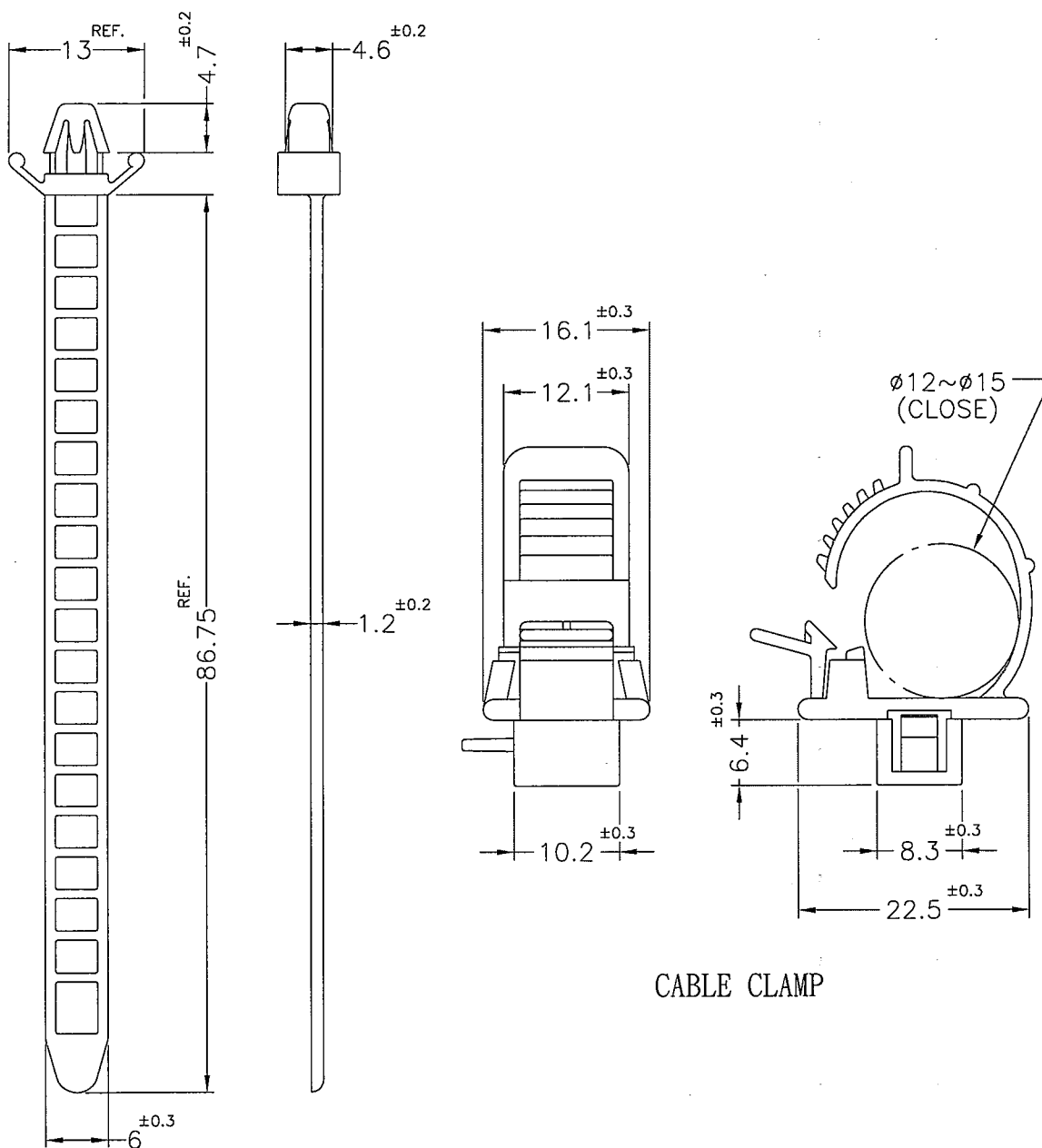
CABLE TIES
