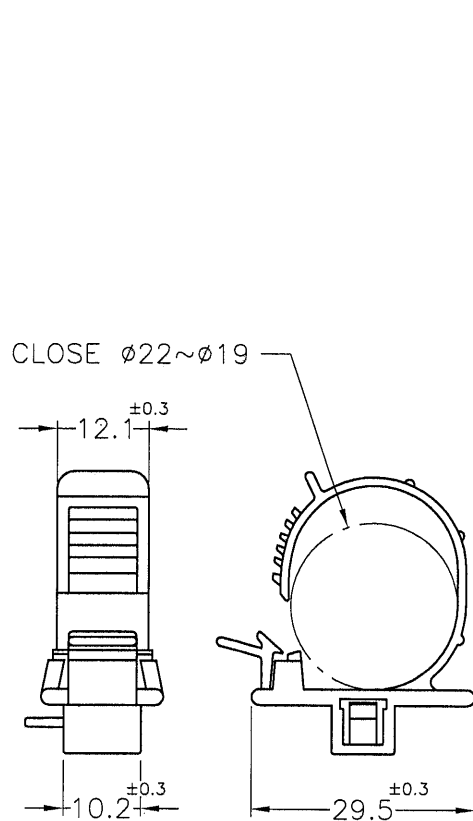
CABLE CLAMP
