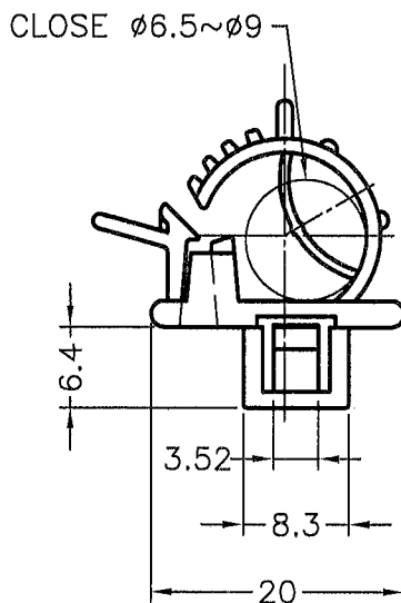
WIRE MOUNT
