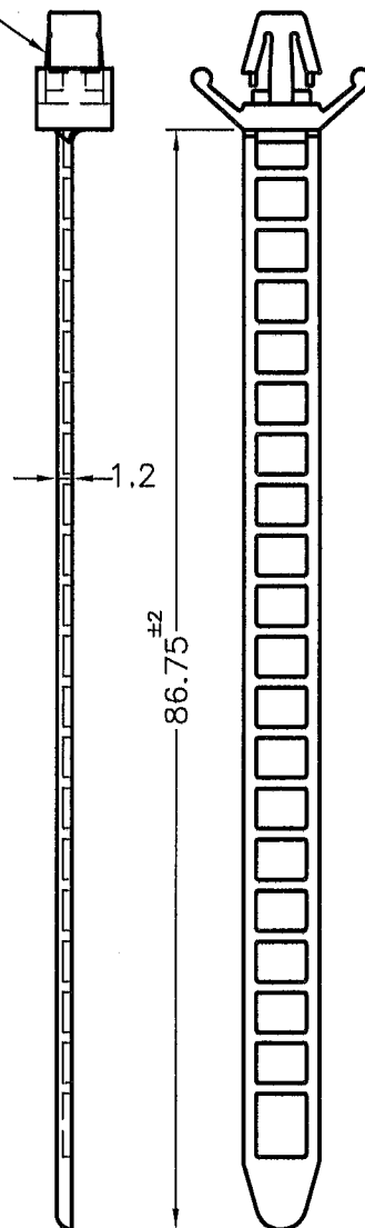
CABLE TIES
