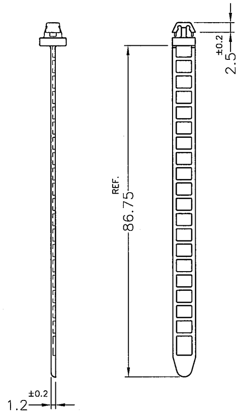
CABLE TIES
