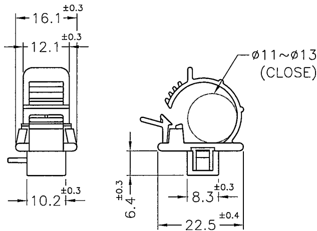
CABLE CLAMP
