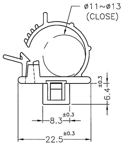
CABLE CLAMP
