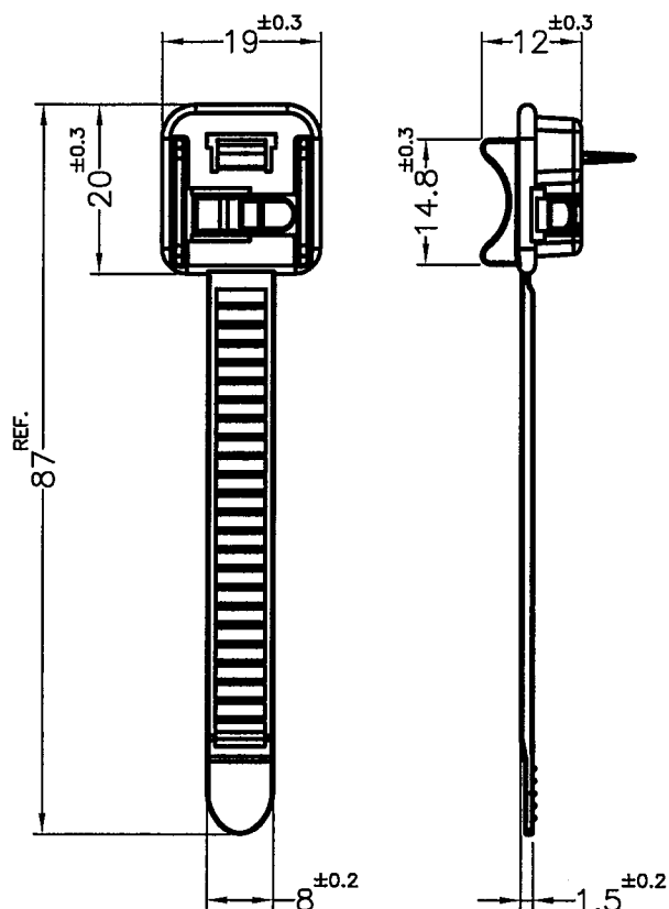
CABLE CLAMP
