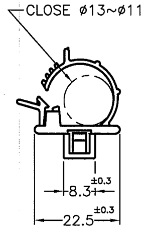
CABLE CLAMP
