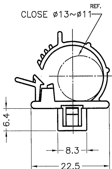
CABLE CLAMP
