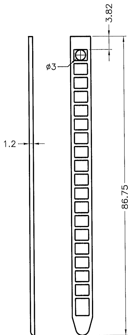
CABLE TIES
