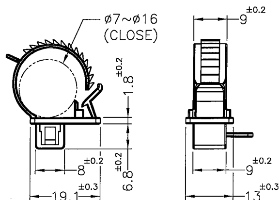
CABLE CLAMP
