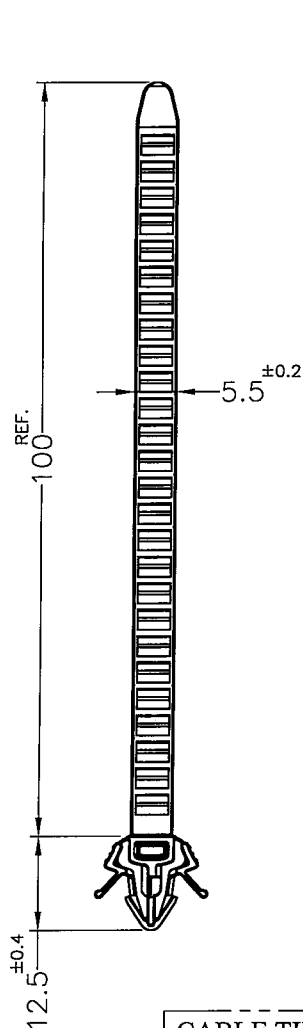
CABLE TIES
