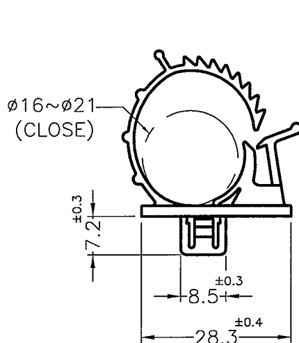
CABLE CLAMP
