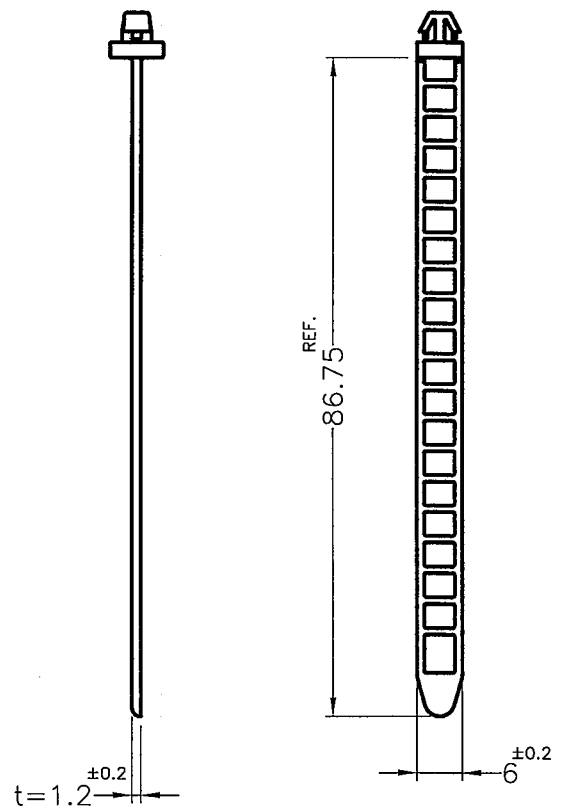
CABLE TIES
