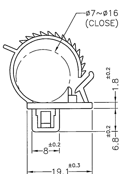
CABLE CLAMP
