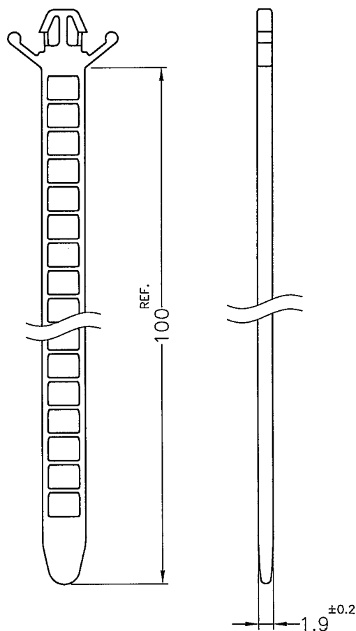
CABLE TIES
