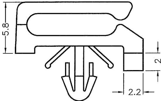
MOUNTING HOLE \phi 3 CHASSIS THICKNESS 1.0~2.2
