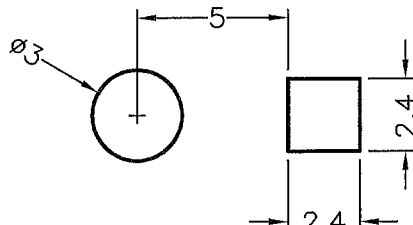
MOUNTING HOLES
