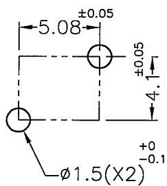
MOUNTING HOLE
