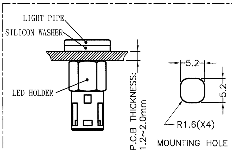
Installation Diagram (Cargo issued without assembly)
