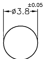
RECOMMEND HOLE IN P.C.B
