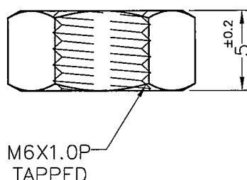
NUT NYLON 66 UL94V-2 COLOR: NATURAL
