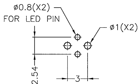
MOUNTING HOLE
