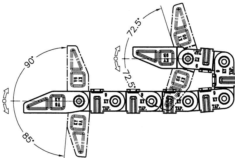
PRINCIPLE SKETCH - BEND RA-DIUS
