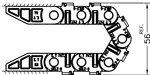
PRINCIPLE SKETCH - BEND RA-DIUS
