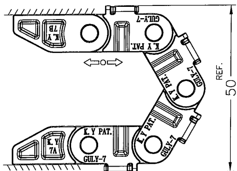
PRINCIPLE SKETCH - BEND RA-DIUS
