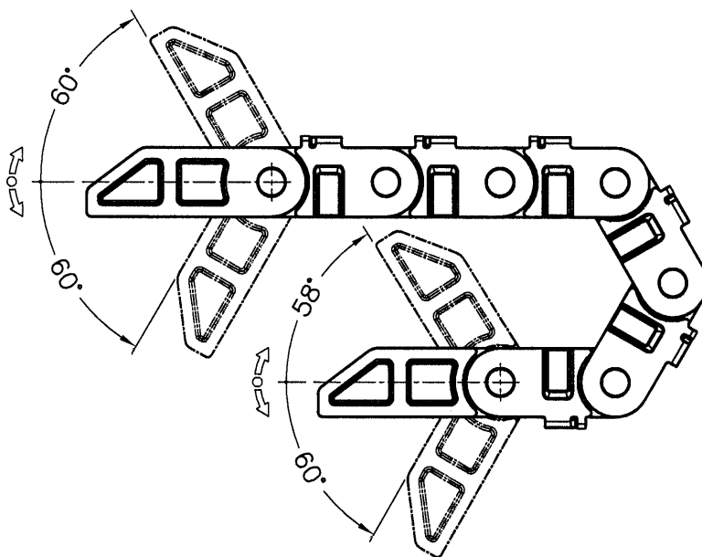
PRINCIPLE SKETCH - BEND RA-DIUS
