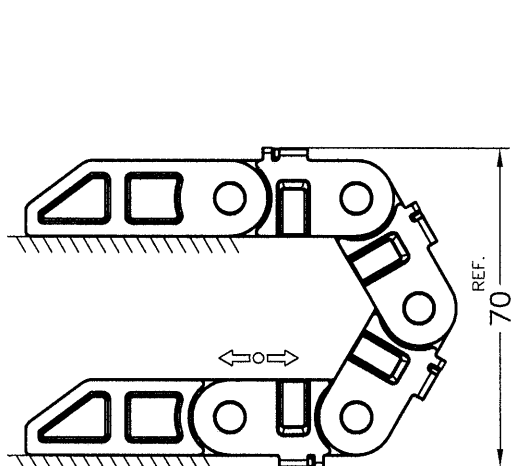
PRINCIPLE SKETCH - BEND RA-DIUS
