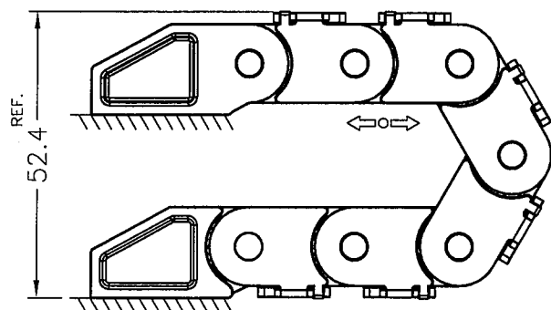
PRINCIPLE SKETCH - BEND RA-DIUS
