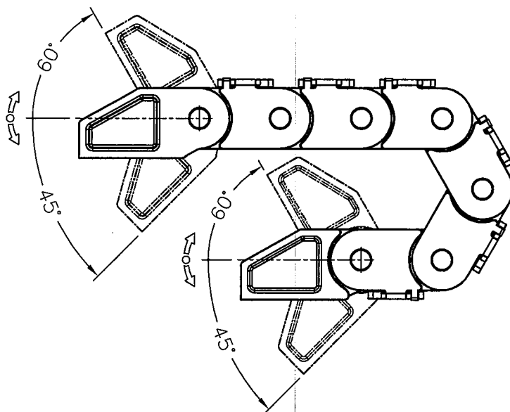
PRINCIPLE SKETCH - BEND RA-DIUS
