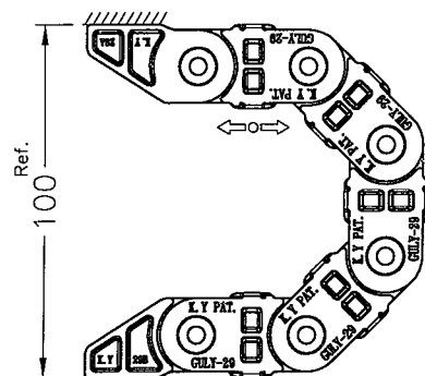
PRINCIPLE SKETCH-BEND RA-DIUS
