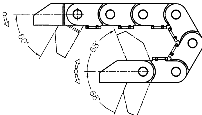
PRINCIPLE SKETCH - BEND RA-DIUS
