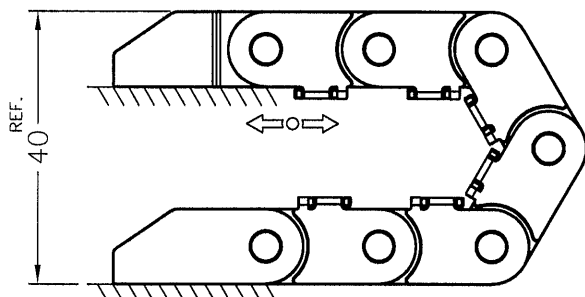
PRINCIPLE SKETCH - BEND RA-DIUS
