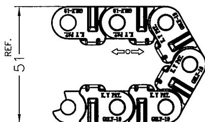
PRINCIPLE SKETCH - BEND RA-DIUS
