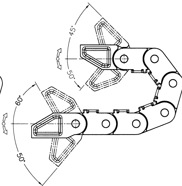
PRINCIPLE SKETCH - BEND RA-DIUS
