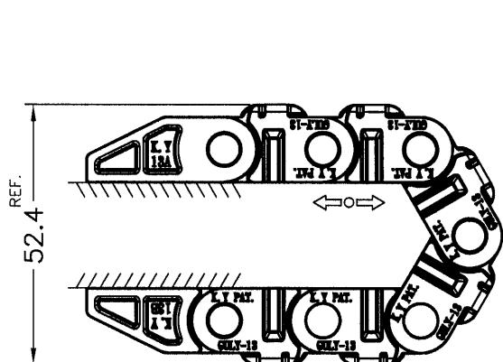
PRINCIPLE SKETCH - BEND RA-DIUS
