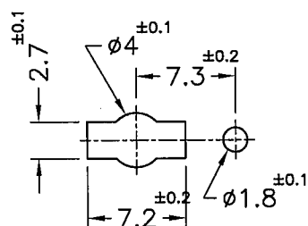
MOUNTING HOLE CHASSIS THICKNESS 0.8~1.6mm
