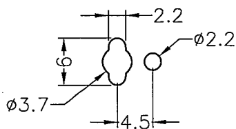
MOUNTING HOLE
