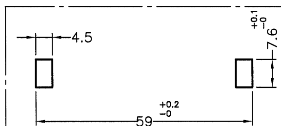
MOUNTING HOLE
