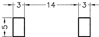
MOUNTING HOLES
