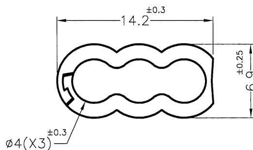
CLOSE VIEW (扣合示意圖)
