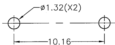
RECOMMENDED MOUNTING HOLE PARTERN
