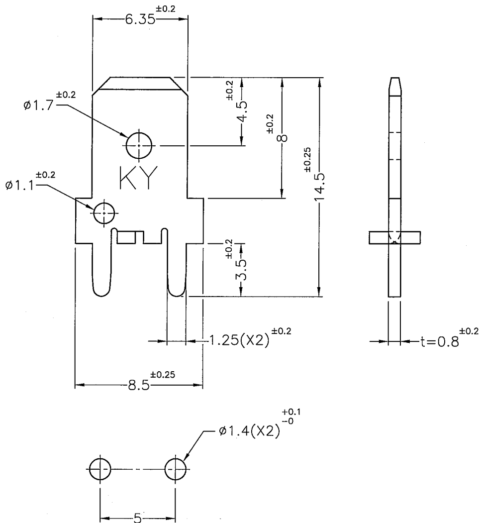
MOUNTING HOLE
