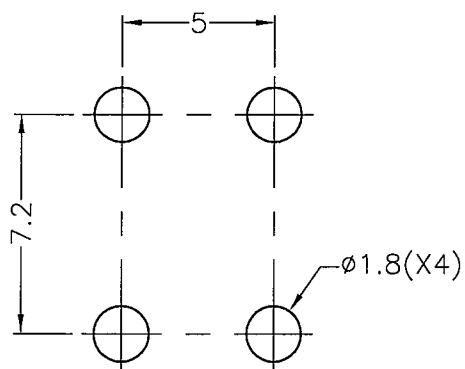
MOUNTING HOLE
