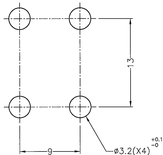
MOUNTING HOLE
